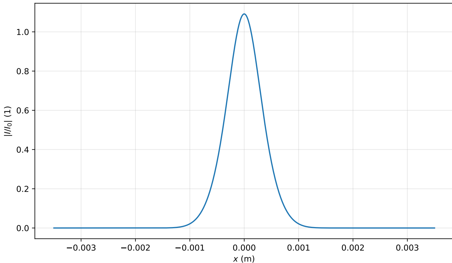
Intensity profile I(x, y = 0, z = 0.637m)/I_0 , P_{in}=0.6P_{cr} , artificial time
